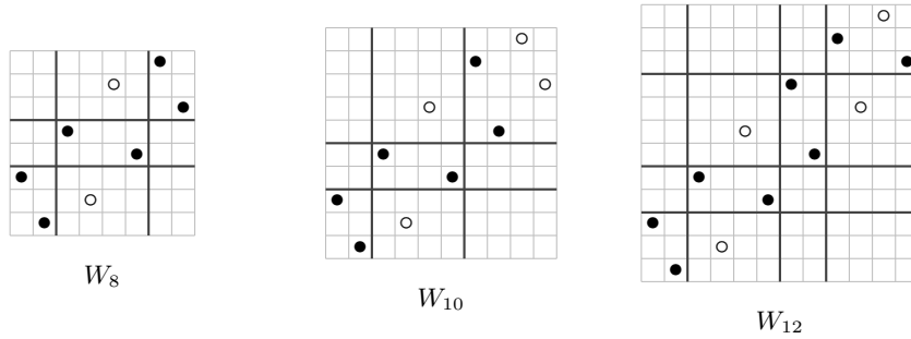
Figure 5: Examples of unused points when embedding \oplus^r 21 .
