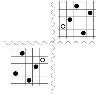
Figure 6: The intervals 25134 and 23514 in Theorem 15. Normal embeddings may omit some of the hollow points.
