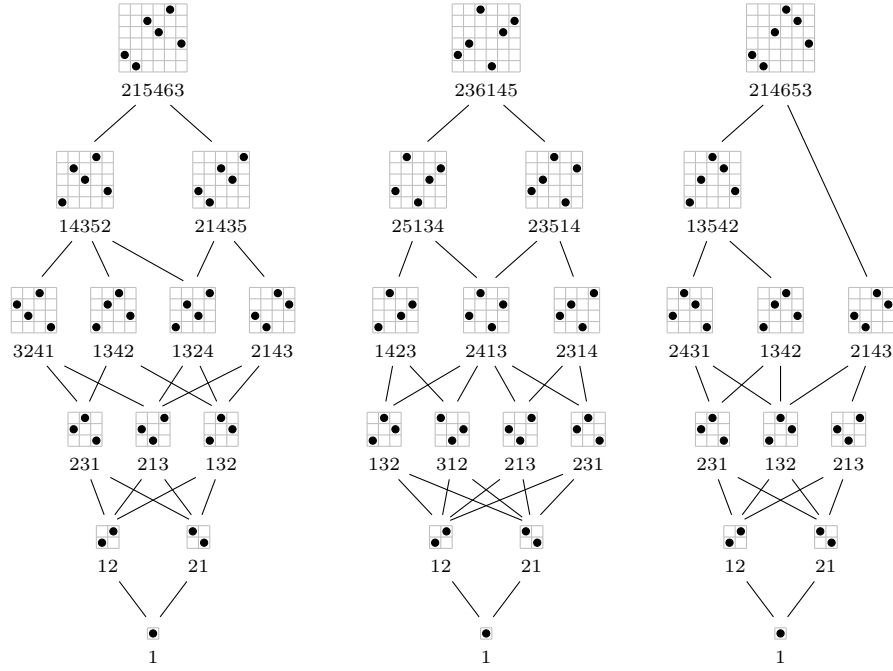
Figure 7: The three annihilators from Theorem 16, and the posets of their subpermutations. The figures omit the permutations with opposing adjacencies, as well as the permutations with an interval copy of a permutation of the form \alpha \oplus 1 \oplus \beta .
