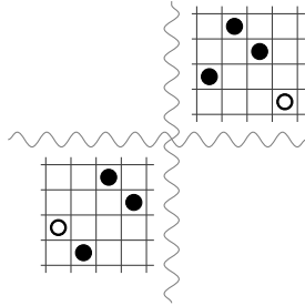
Figure 4: The intervals 2143 and 2431 in Theorem 13. Normal embeddings may omit some of the hollow points.
