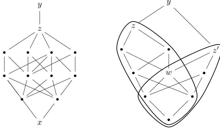
Figure 2: Examples of narrow-tipped (left) and diamond-tipped (right) posets.
